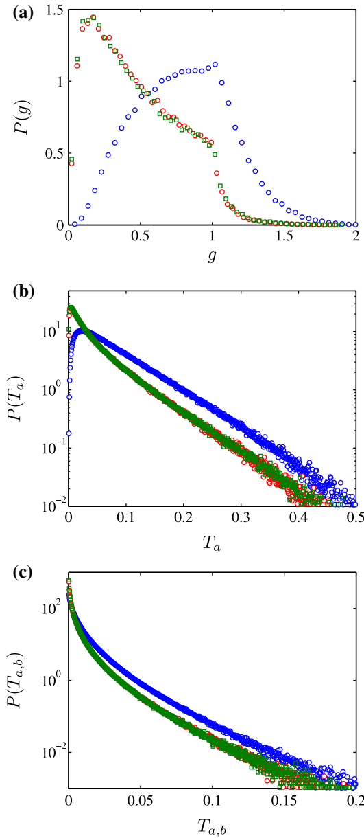
Figure 3. (Color online) Panel (a) shows the distribution of dimensionless conductance P(g) for three waveguides, each with 10 propagating channels. P(g) from the numerical simulation of waveguide with length L/\lambda = 200 and no evanescent channels, blue open circles, is significantly distinct from P(g) for the same geometry and N_e = 8 evanescent channels, green squares. However, the system with evanescent channels is equivalent to a longer system, L'/\lambda = 300 , with an equivalent value of L/\lambda - red open circles. Hence, the only effect of inclusion of evanescent channels is to renormalize \ell(N_e) . Panels (b,c) demonstrate that this argument also applies to P(T_a) and P(T_{ab}) , respectively.
