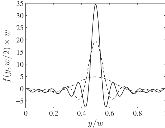
Figure 1. Random potential f(y, y_m) with y_m = w/2 is reconstructed from Equation (6) using the procedure described in the Appendix. Dot-dash, dash, and solid lines correspond to N_p + N_e = 2, 6, 10 respectively. One can observe the convergence of f(y, y_m) \rightarrow \delta(y - y_m) with an increase in N_p + N_e .
