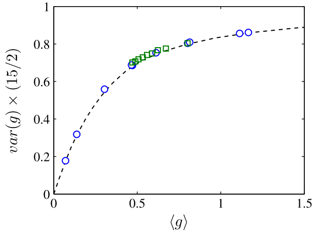
Figure 2. (Color online) Variance of dimensionless conductance is plotted vs. its mean value. Open circles represent numerically computed data for systems with N_p = 10 , N_e = 0 and varying L . The dashed line plots Equation (6.23) of Ref. [44], derived using the supersymmetry approach. No fitting parameters are used. As per single parameter scaling (SPS), the variance of dimensionless conductance is uniquely determined by its average. Open squares represent the system with L/\lambda = 200 , N_p = 10 and N_e from 0 to 8 evanescent channels in the right-to-left order. The effect of evanescent channels is to effectively reduce \langle g \rangle or, in other words, to renormalize (decrease) \ell(N_e) while retaining the property of SPS.
