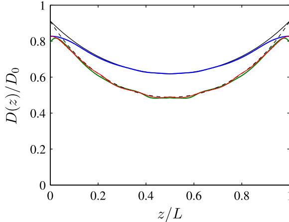
Figure 4. (Color online) (a) Position-dependent diffusion coefficient D(z)/D_0 for the three geometries shown in each of the panels in Figure 3. The diffusion coefficient for two microscopically different samples ( N_e = 8 – green and N_e = 0 – red solid lines) coincides because they both have identical value of L/\ell hence confirming the universality of D(z) . The result of SCT is shown as solid and dashed black lines for two values of L/\ell . Numerical simulations and SCT agree without fitting in both cases with exception of two boundary regions.
